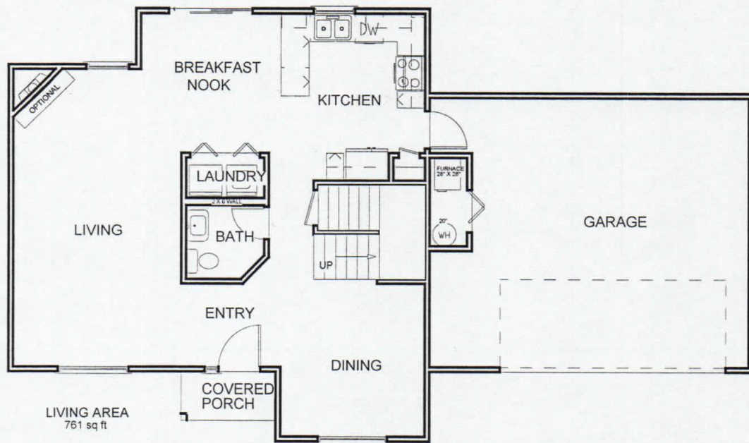
FIRST FLOOR
